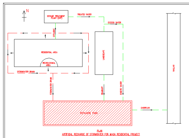
Figure 1. The schematic plan of recharge structure.
