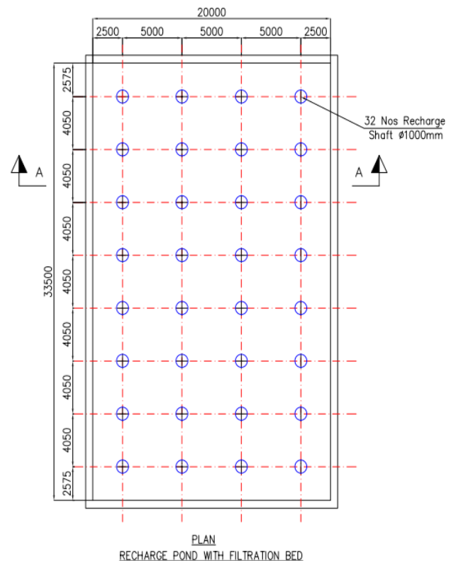
Figure 2. Schematic diagram of recharge pond with filtration bed.
