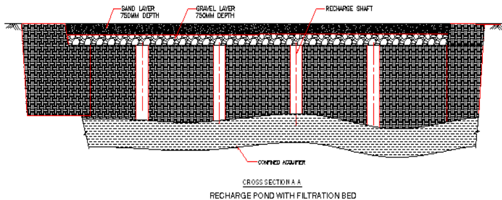
Figure 3. Cross section of recharge pond with shaft.
