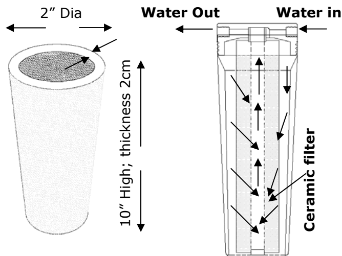
Fig. 3. Coated plain ceramic cartridge Inner side covered with a sediment filter
