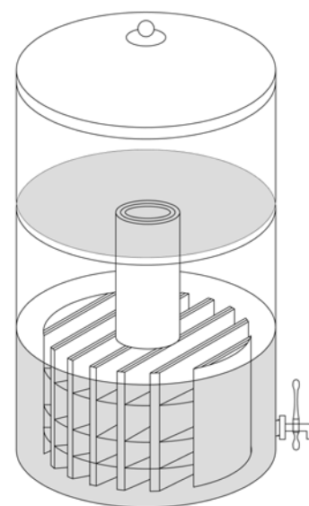
Fig. 14. Nano silver disinfection: water purifier assembly view
