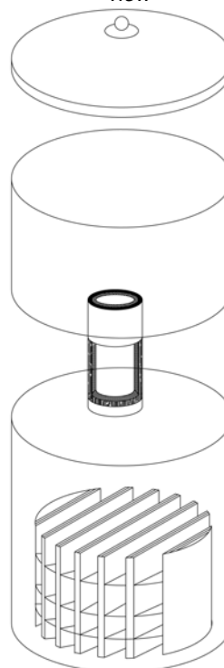
Fig. 13. Nano silver disinfection: water purifier components split view
