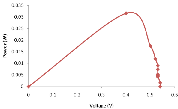
(b) P-V Curve
