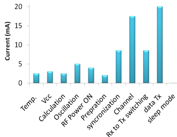
Figure 6. Current Consumption with Different Tasks.
