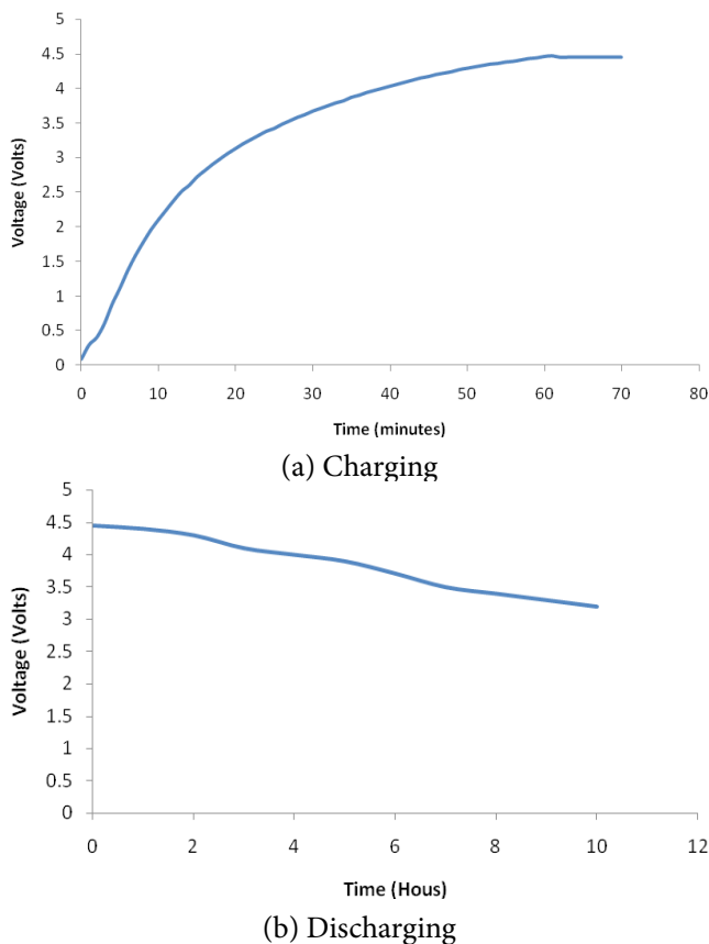
Figure 8. Supercapacitor Characteristics (a) Charging (b) Discharging.
