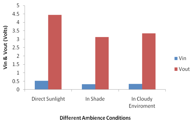
(b) Experimental Input and Output Voltages
