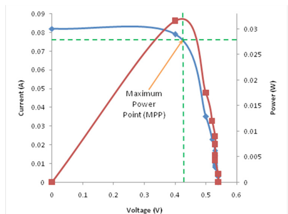
(c) Maximum Power Point Curve
