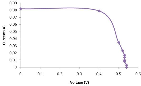
(a) I-V Curve
