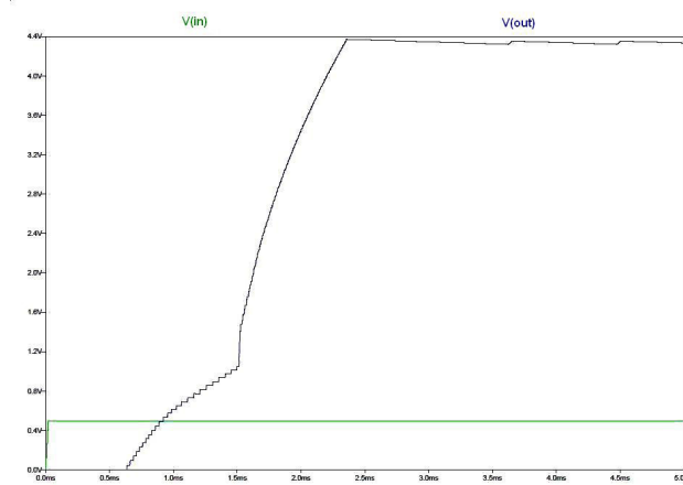
(a) Simulation Input and Output Voltages
