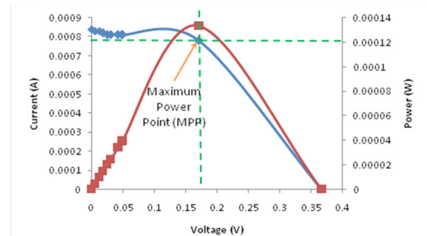
(c) Maximum Power Point Curve
