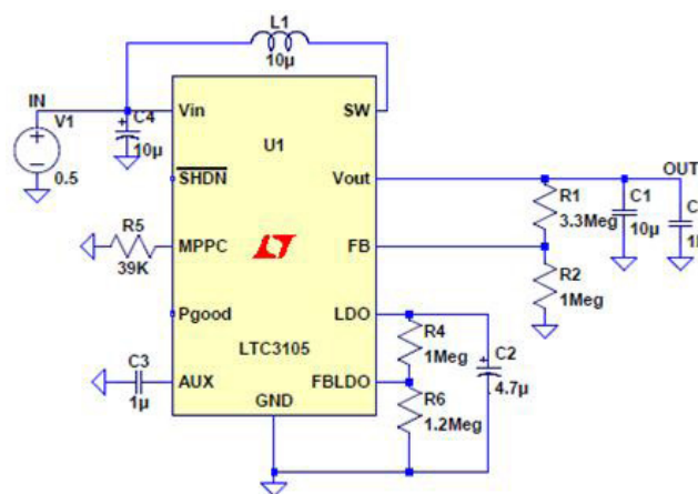
Figure 2. Schematic Diagram of Energy Scavenging Interface Circuit.
