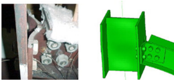
Figure 4. Comparison of simulation and observed deformation patterns of web connection.
