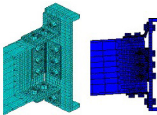
Figure 3. Deformed shape of connection.
