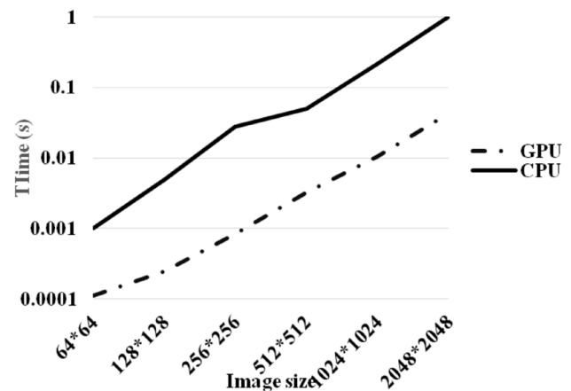
Figure 7. The simulation results for images with different resolutions by Cuda C++ C++ and Visual C++.
