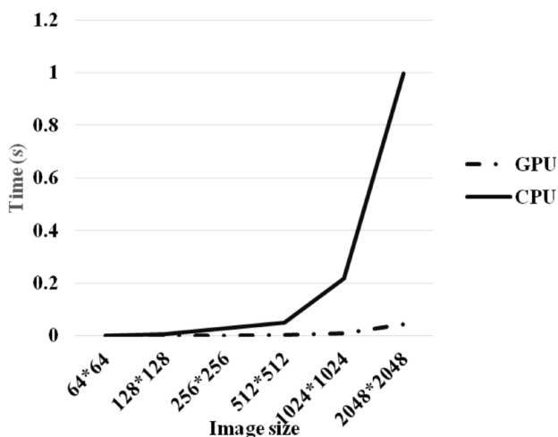
Figure 6. The simulation results for images with different resolutions by Cuda C++ C++ and Visual C++.
