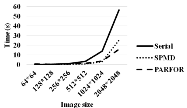
Figure 8. The simulation results for images with different resolutions by MATLAB and its parallelism methods.
