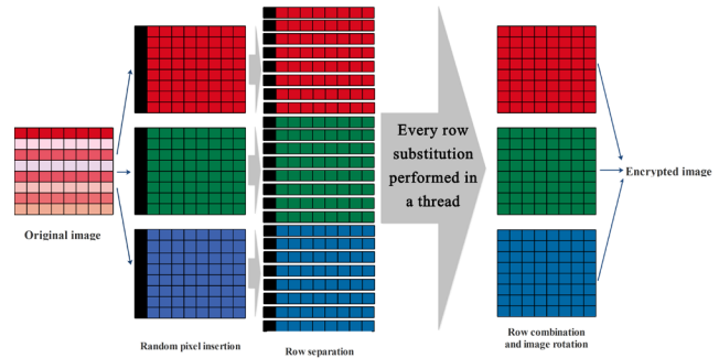
Figure 5. Implementation of one round of the 1D chaos-based image encryption algorithm using CUDA C++.
