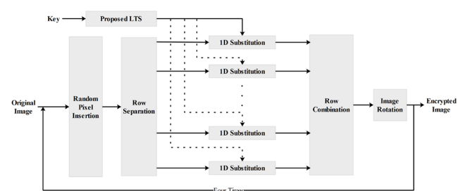
Figure 2. 1D chaos-based image encryption algorithm.
