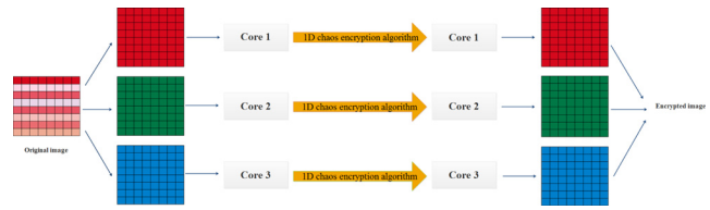
Figure 4. Implementation of one round of the 1D chaos-based image encryption algorithm using SPMD.
