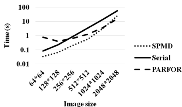
Figure 9. The simulation results for images with different resolutions by MATLAB and its parallelism methods.
