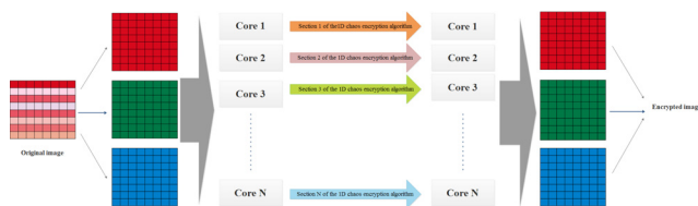
Figure 3. Implementation of one round of the 1D chaos-based image encryption algorithm using PARFOR.
