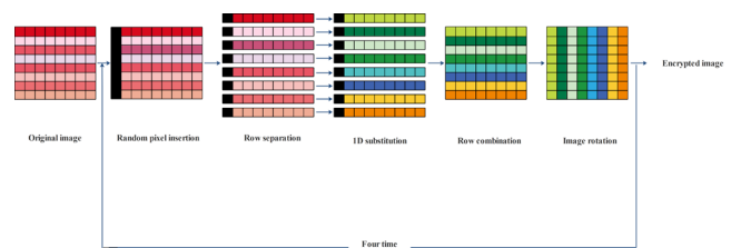
Figure 1. An example of the 1D chaos-based image encryption algorithm.
