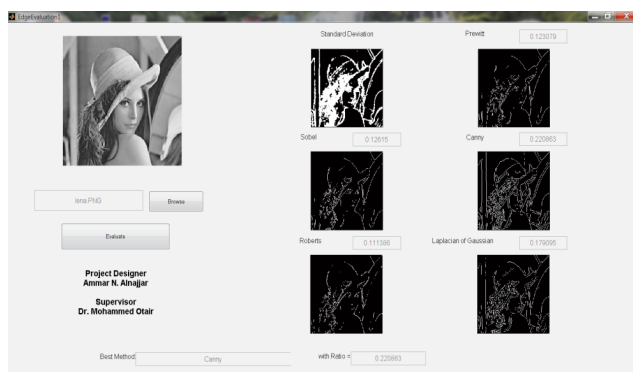
Figure 3. The Final GUI Results for Lena Image.
