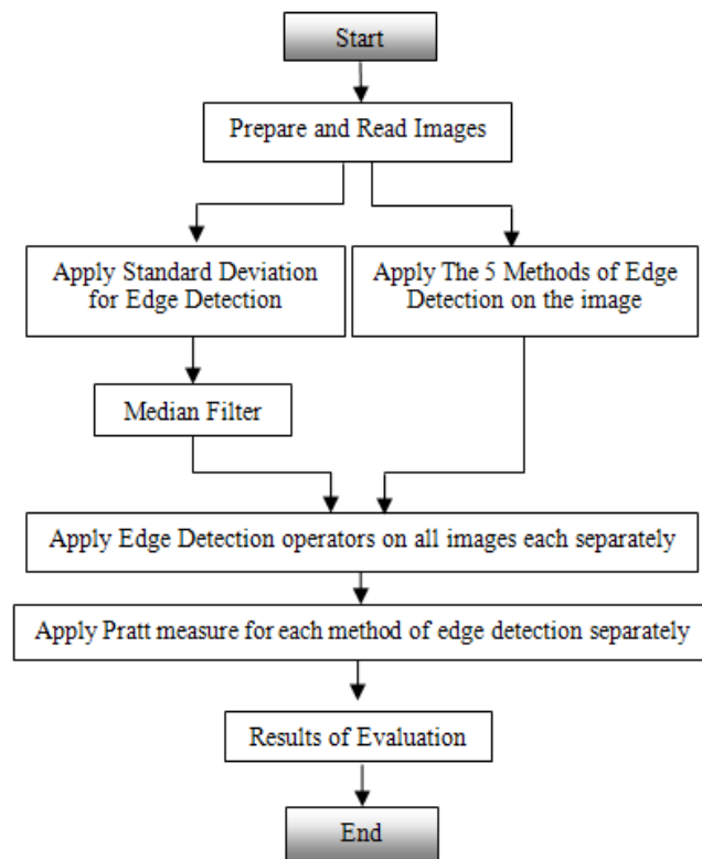
Figure 1. The Work Flow Diagram of A-EDV.
