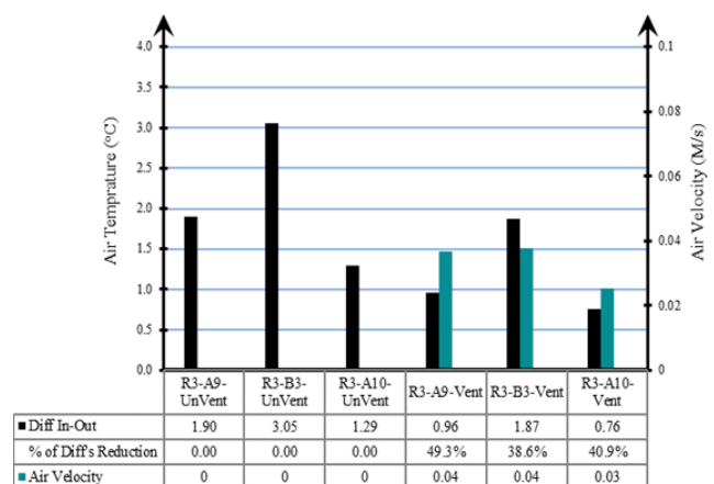
Figure 16. Air temperature reduction with reference to air velocity in ventilated and unventilated R3 rooms (night-time).
