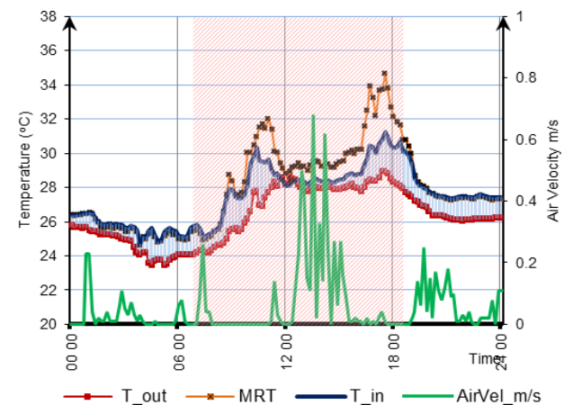
Figure 12. Room (A10) ventilated on 14 July 09.
