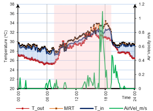
Figure 10. Room (B3) ventilated on 9 June 09.
