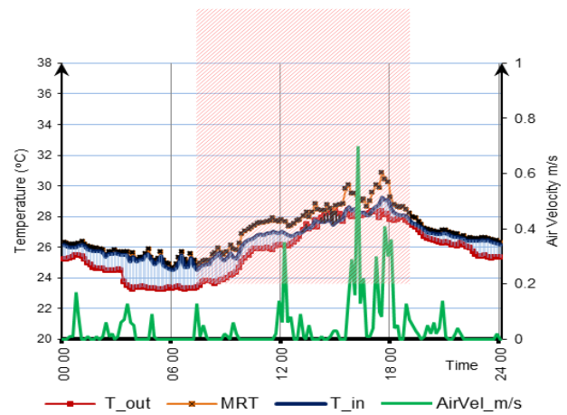
Figure 8. Room (A9) ventilated on 21 April 09.
