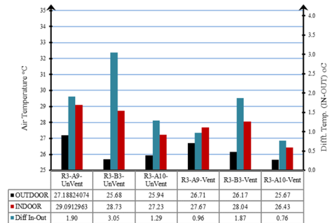
Figure 14. Summary of average air temperature in ventilated and unventilated R3 rooms (night-time)..
