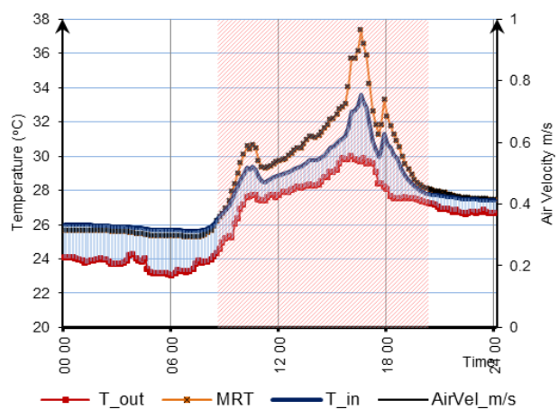
Figure 11. Room (A10) unventilated on 13 July 09.
