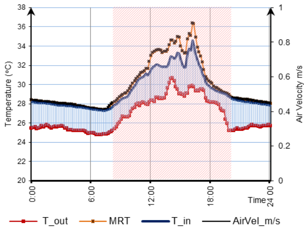
Figure 7. Room (A9) unventilated on 13 April 09..
