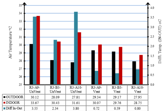
Figure 13. Summary of average air temperature in ventilated and unventilated R3 rooms (daytime).
