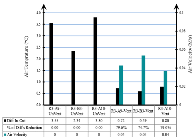
Figure 15. Air temperature reduction with reference to air velocity in ventilated and unventilated R3 rooms (daytime).
