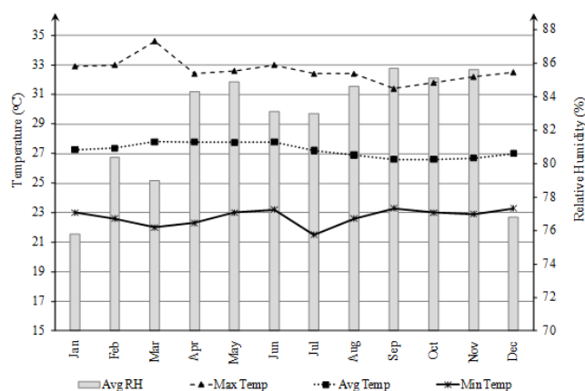
Figure 2. Maximum, minimum, and average dry bulb temperature and average relative humidity in Penang.
