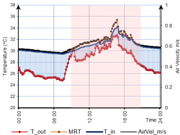
Figure 9. Room (B3) unventilated on 7 June 09.
