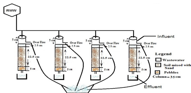
Figure 1. Schematic illustration of the soil columns setup.
